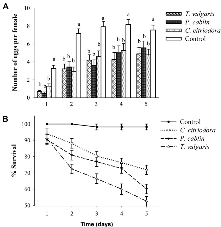
Fig. 4. Mean ( \pm SE) number of eggs per female (A) and female survival (B) for five days of Bemisia tabaci after feeding on the plants treated by 0.5% essential oils under no-choice condition. Bar heads with different letters in each cluster indicate significant differences (HSD test; P < 0.01 ) of egg/female/day among treatments.
