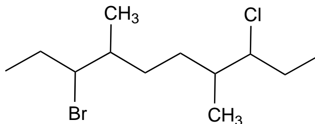
3-bromo-8-chloro-4,7-dimethyldecane
