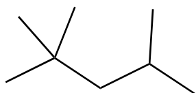
2,2,4-trimethylpentane
