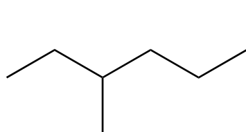
3-methylhexane
