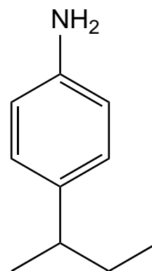
4- sec -butylaniline
