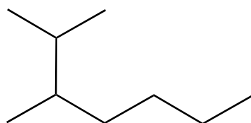
2,3-dimethylheptane
