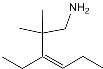
3-ethyl-2,2-dimethyl-3-hexen-1-amine
