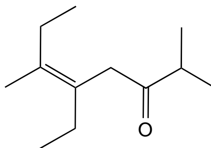
5-ethyl-2,6-dimethyl-5-octen-3-one
