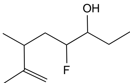
4-fluoro-6,7-dimethyl-7-octen-3-ol
