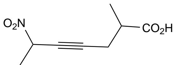
2-methyl-6-nitro-4-heptynoic acid
