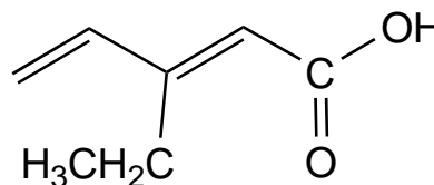
3-ethyl-2,4-pentadienoic acid
