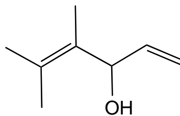
4,5-dimethyl-1,4-hexadien-3-ol
