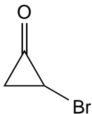
2-bromocyclopropanone
