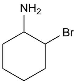
2-bromocyclohexanamine
