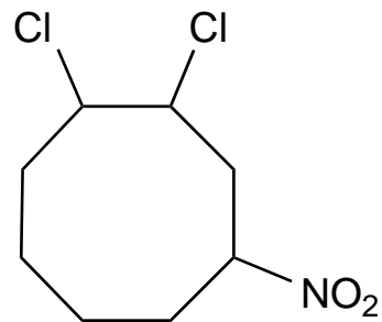
1,2-dichloro-4-nitrocyclooctane
