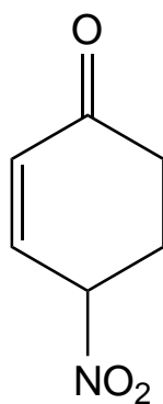
4-nitro-2-cyclohexenone
