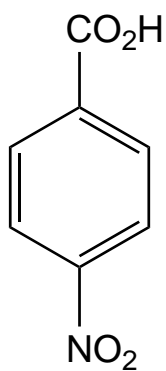
4-nitrobenzoic acid
