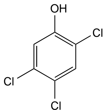
2,4,5-trichlorophenol
