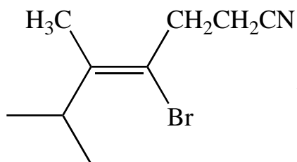
Z -4-bromo-5,6-dimethyl-4-heptenenitrile
