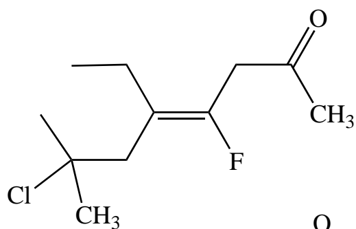
Z -7-chloro-5-ethyl-4-fluoro-7-methyl-4-octen-2-one
