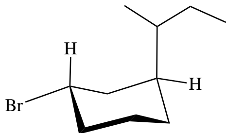
trans -1-bromo-3-sec-butylcyclohexane
